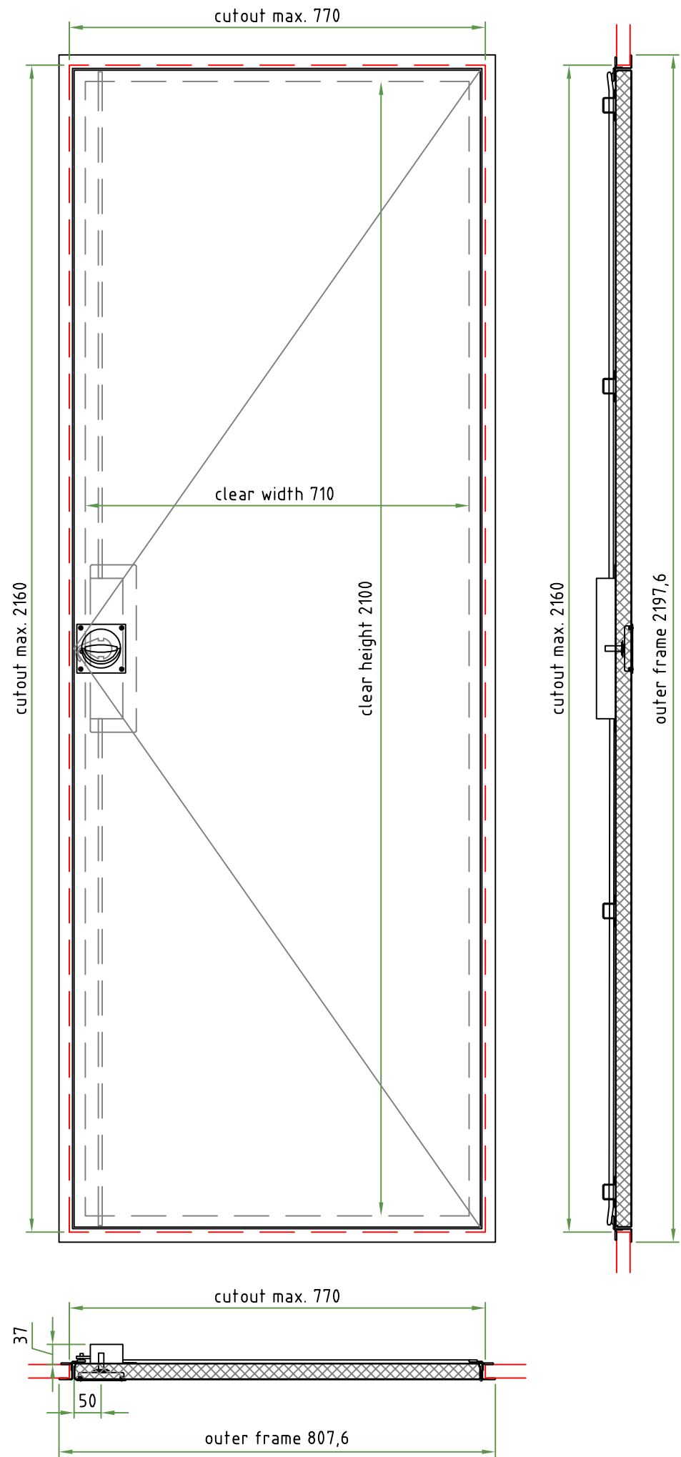
ID6-B15 - max. dimensions shell type handle M 1:10
