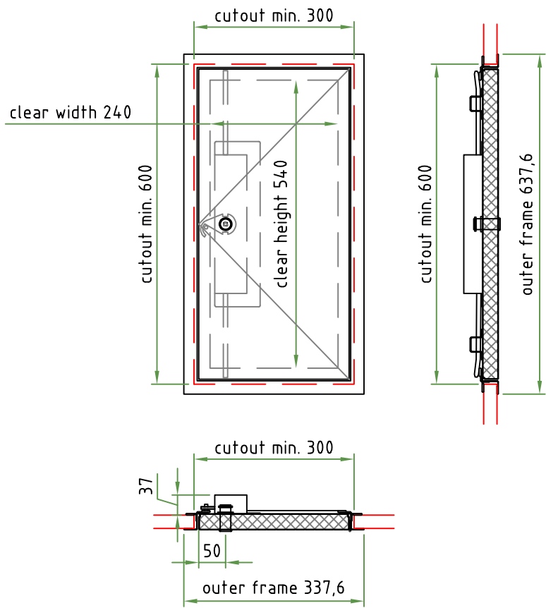
ID6-B15 - min. Dimensions triangular / square lock M 1:10
