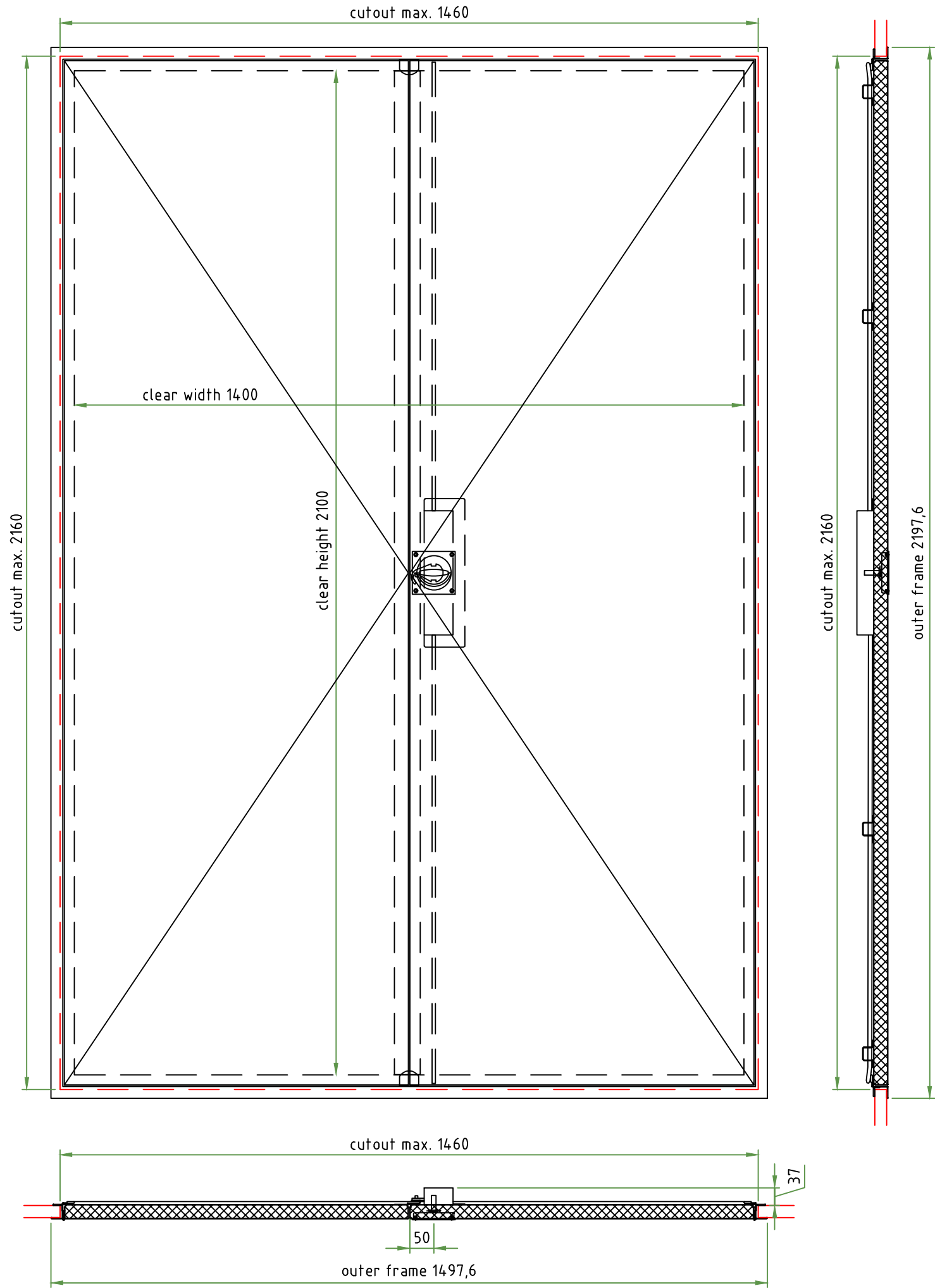
ID5-B15 - max. dimensions shell type handle M 1:10
