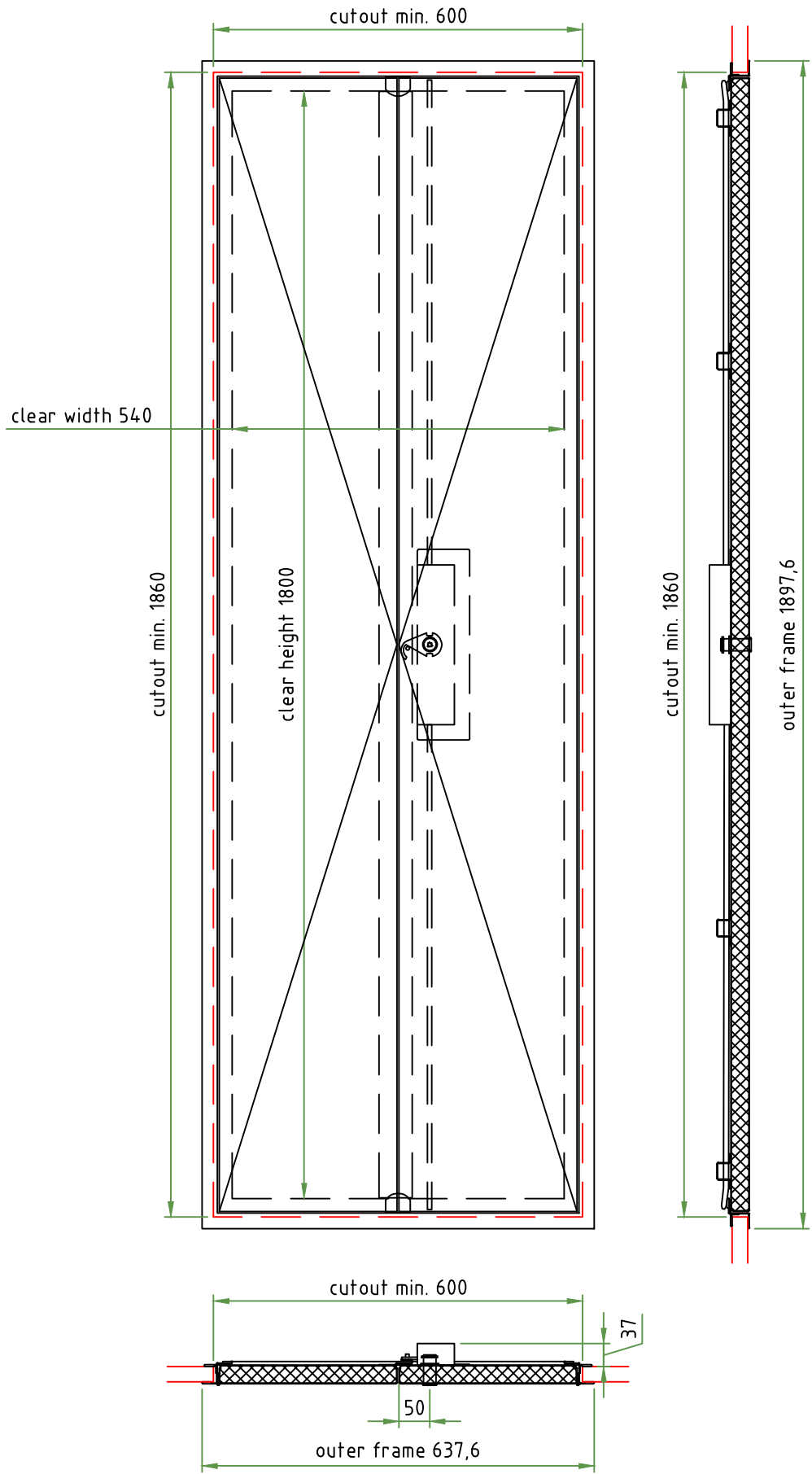
ID5-B15 - min. dimensions triangular / square lock M 1:10
