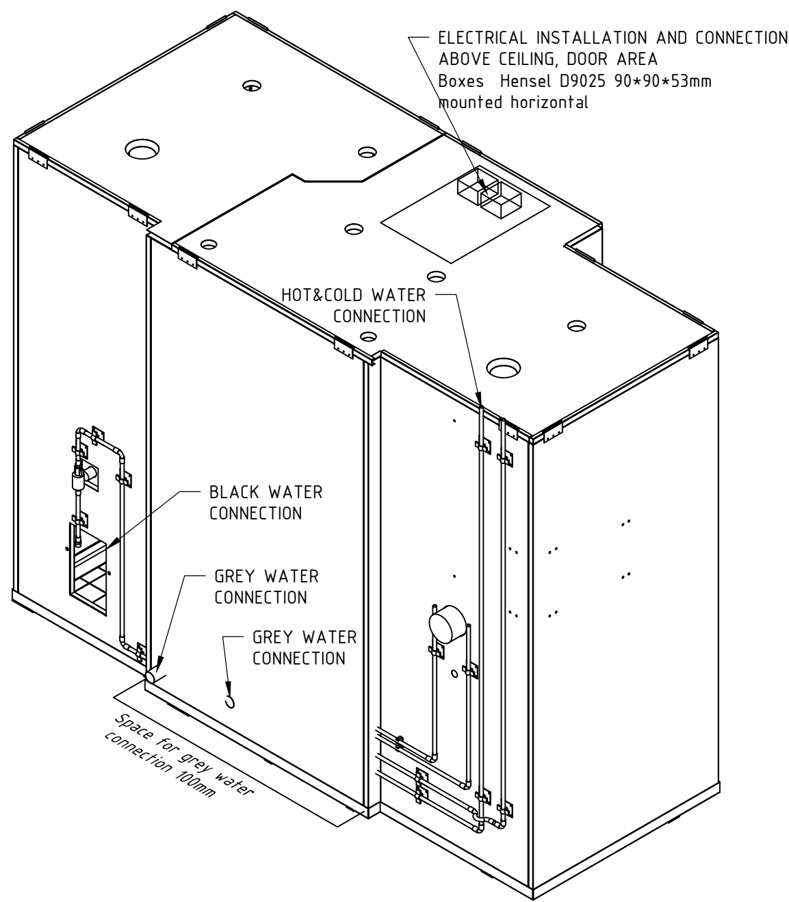
Wet Unit Type C - ISO Connections
