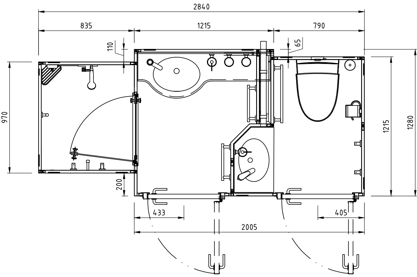
Wet Unit Type C - Floorplan
