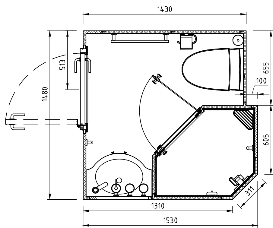
Wet Unit Type D - Floorplan
