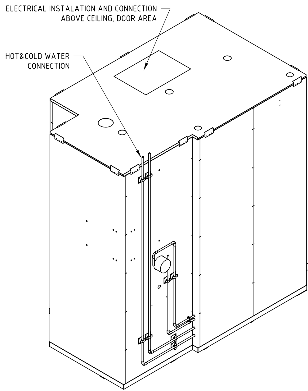
Wet Unit Type B - ISO Connections
