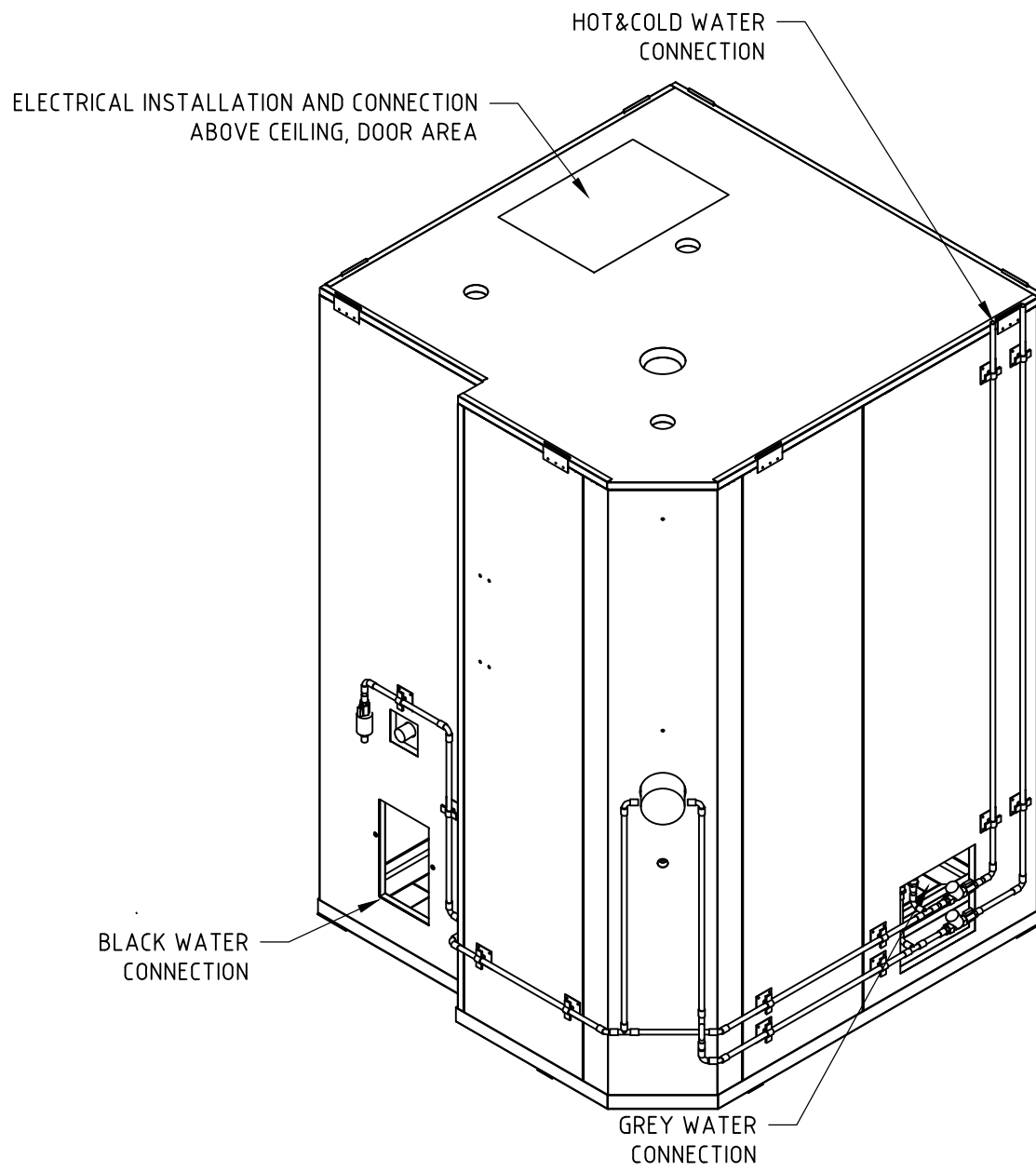
Wet Unit Type D - ISO Connections
