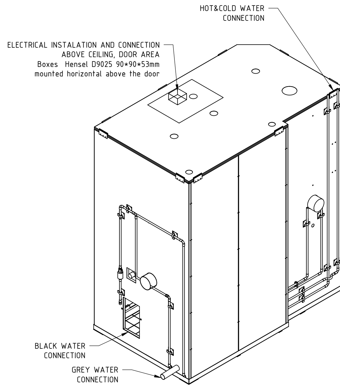
Wet Unit Type A - ISO Connections
