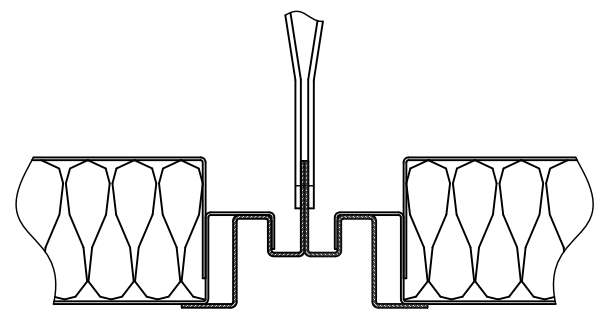
Support profile alternative D for LM40 ceiling sytem only
