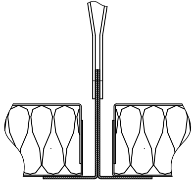
Support profile alternative A
