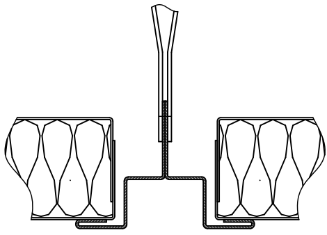
Support profile alternative C
